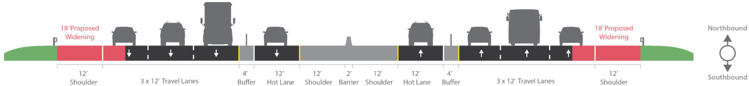
I-664 : 6GP + 2 M I-664 Tunnel Split to Powhatan Parkway Interchange
