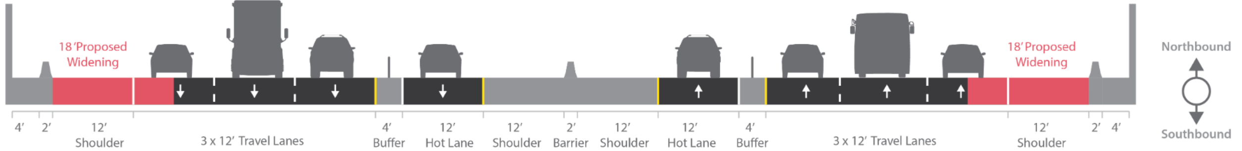
I-664 : 6GP + 2 M I-664 Tunnel Split to Powhatan Parkway Interchange
