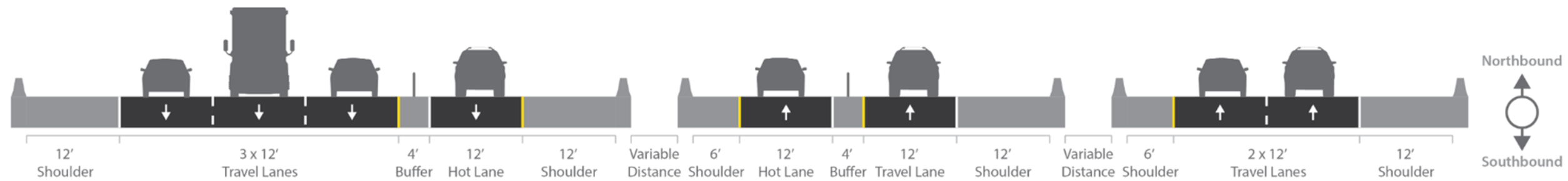
Bridge and Tunnel Across Hampton Roads North of I-664 Connector: 6 GP + 2M
