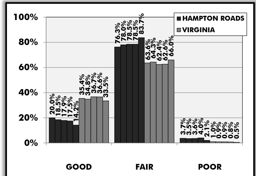
PERCENTAGE OF PAVEMENT IN HAMPTON ROADS AND VIRGINIA BY CONDITION NON-INTERSTATE NHS (2017 - 2021)
