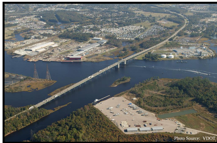
I-64, High-Rise Bridge over the Southern Branch of the Elizabeth River in Chesapeake, Virginia is projected to carry nearly 1,500 additional trucks each weekday in 20 years
