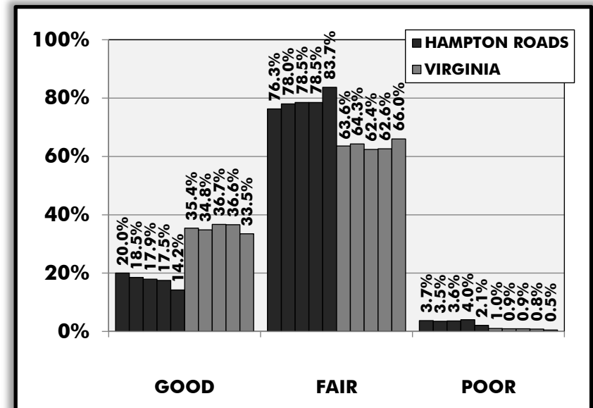
PERCENTAGE OF PAVEMENT IN HAMPTON ROADS AND VIRGINIA BY CONDITION NON-INTERSTATE NHS (2017 - 2021)
