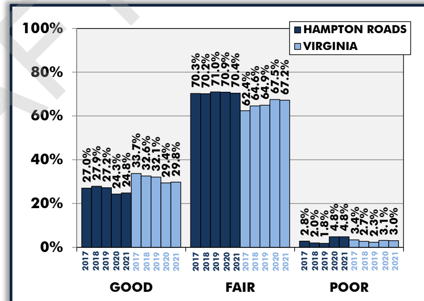
PERCENTAGE OF NHS BRIDGE DECK AREA IN HAMPTON ROADS AND VIRGINIA BY CONDITION (2017 - 2021)
