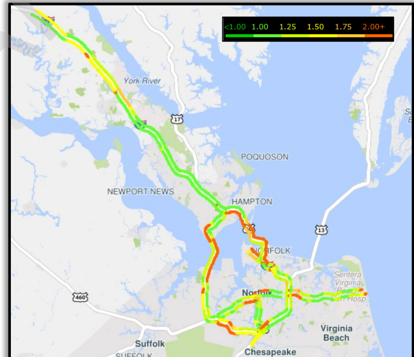
TRUCK TRAVEL TIME RELIABILITY INDEX - INTERSTATE (2021)
