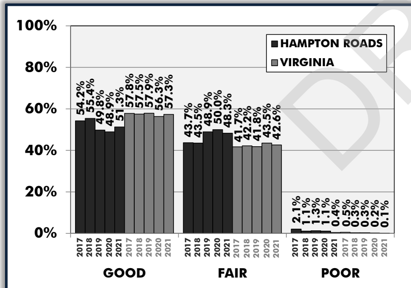
PERCENTAGE OF PAVEMENT IN HAMPTON ROADS AND VIRGINIA BY CONDITION INTERSTATE (2017 - 2021)
