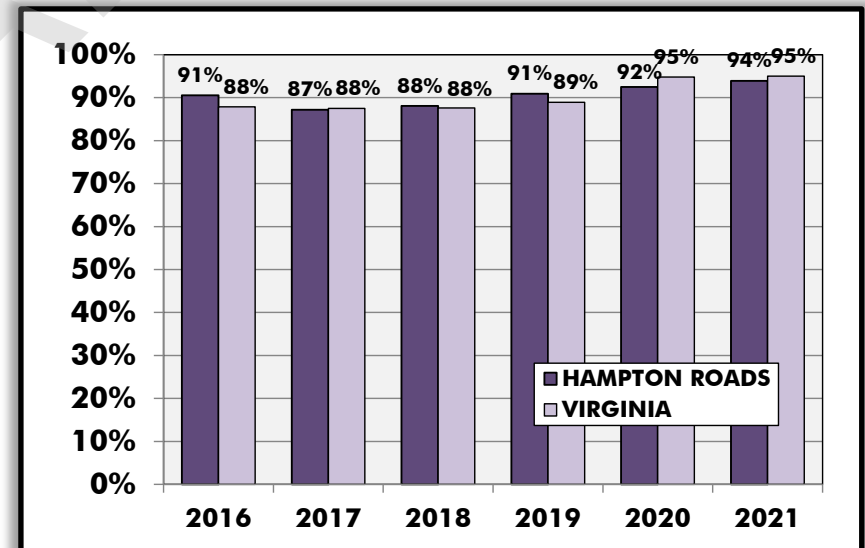
PERCENTAGE OF RELIABLE PERSON-MILES OF TRAVEL - NON-INTERSTATE NHS (2016 - 2021)
