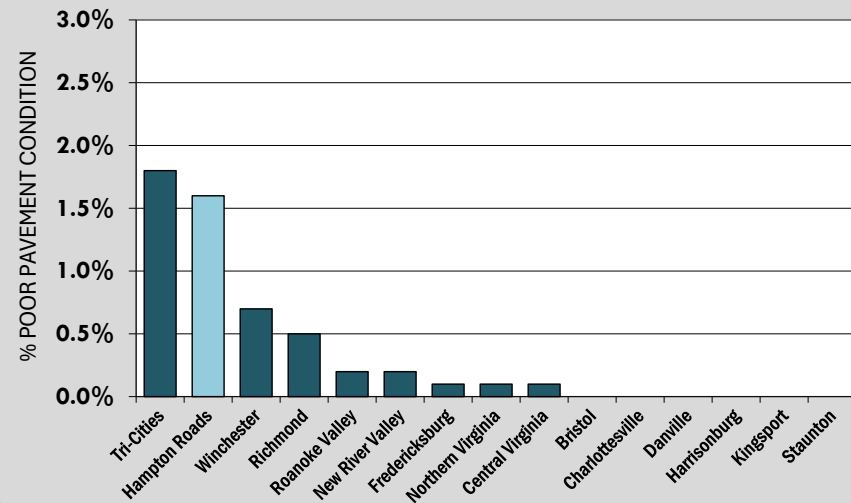
PERCENT OF NON-INTERSTATE NATIONAL HIGHWAY SYSTEM (NHS) PAVEMENT IN POOR CONDITION, 2023
