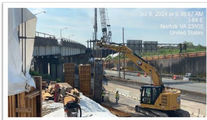
Widening of I-64-EB Bridge over I-564
